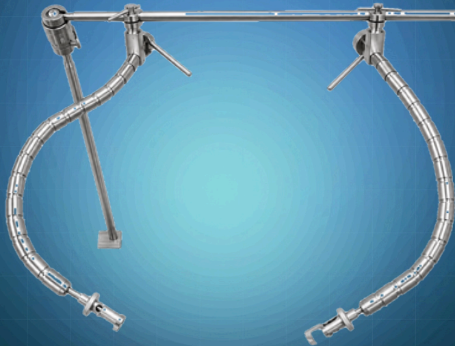
FRAME RETRACTOR
